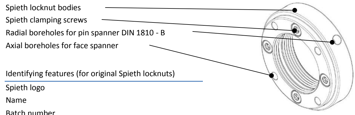
Fig. 1: Schematic representation similar to Spieth MSF series locknuts
