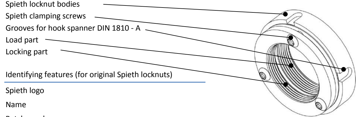
Fig 1: Schematic representation similar to Spieth MSWcompact & MSWperformance series locknuts
