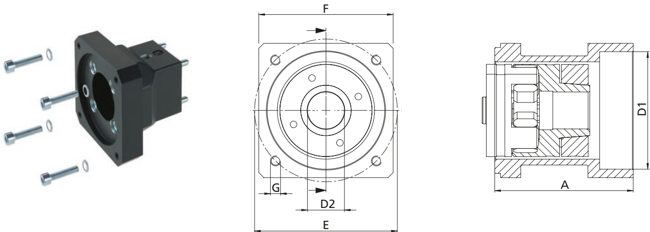
Selection table - motor adaptor/coupling EP(X) -II for three-phase motor
