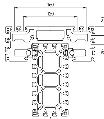
Profile F-80 x 160
